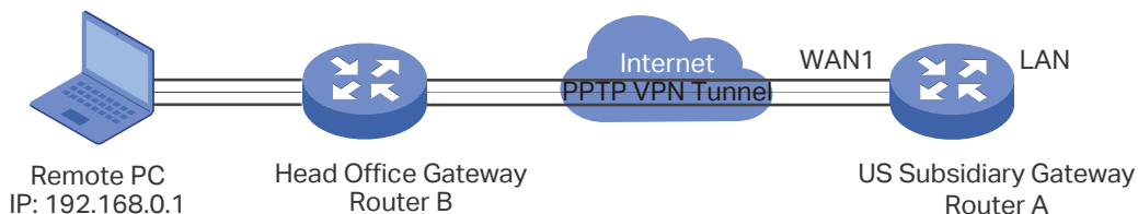
Figure 5-17 Remote Access PPTP VPN Topology
